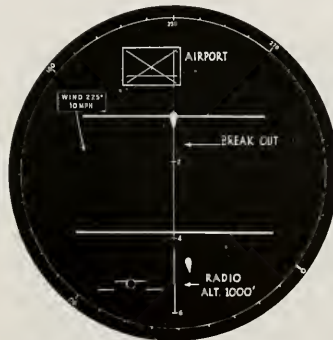
BELOW, LEFT TO RIGHT: FIGURE 2—TYPICAL PICTURE SENT ALOFT BY TELERAN; FIGURE 3—PICTORIAL INSTRUCTIONS WHICH GUIDE PILOT IN LANDING; FIGURE 4—TELERAN WEATHER MAP AND TERRAIN FEATURES. AT RIGHT: FIGURE 5—SUGGESTED METHOD OF MOUNTING TELERAN KINESCOPE IN COCKPIT OF PLANE.
